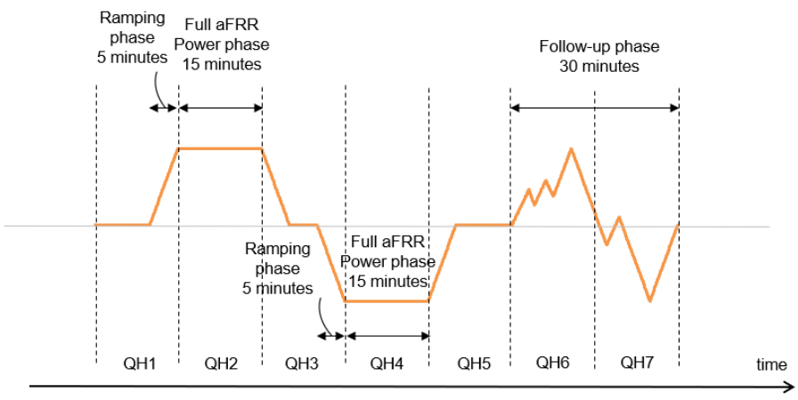
Figure 2 - Prequalification test related to both directions
