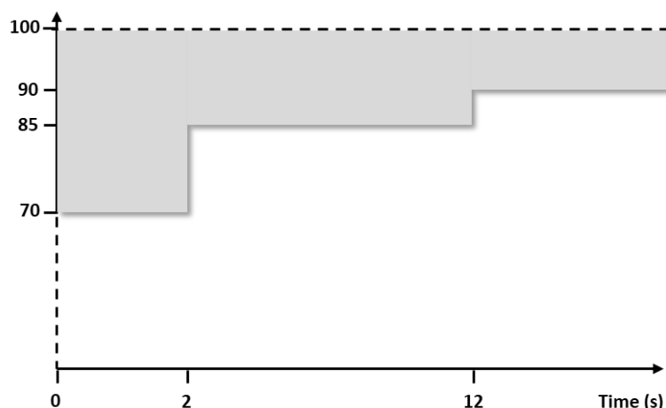
Voltage level (%)
