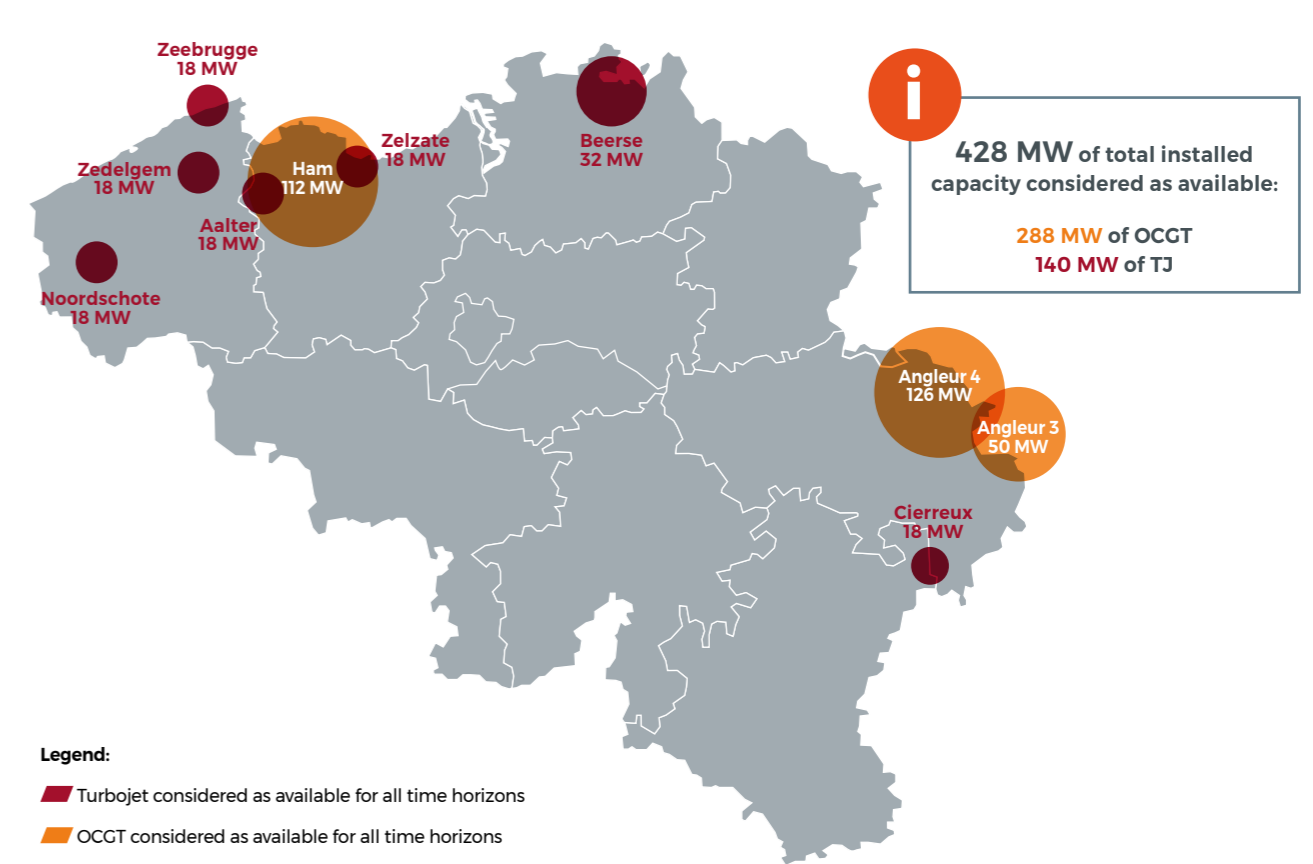
TOTAL INSTALLED OCGT AND TURBOJET CAPACITY AVAILABLE IN BELGIUM [FIGURE 2-27]
