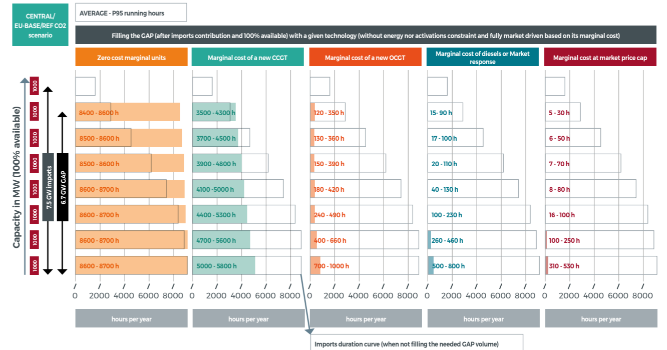
RUNNING HOURS ARE VERY DEPENDENT ON THE TECHNOLOGY CHOICE TO FILL THE IDENTIFIED GAP VOLUME FOR 2025 [FIGURE 4-43]
