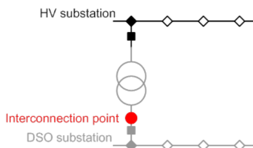
Typical representation of a TSO-DSO interconnection
