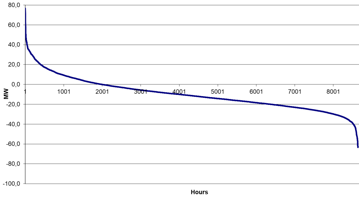
Monotone curve for compensation deficit 2019
