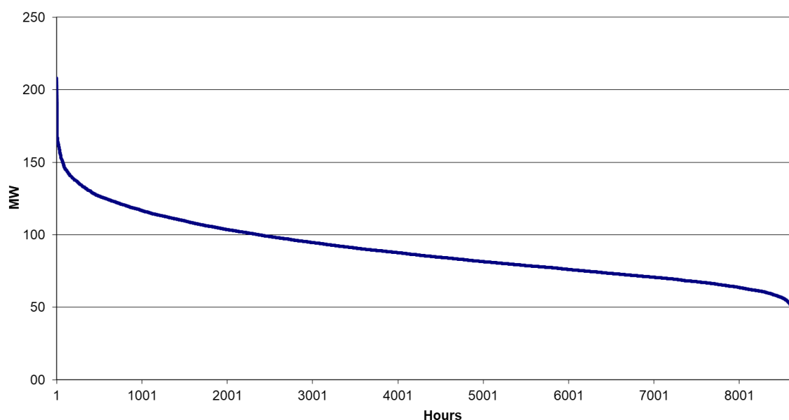
Monotone curve of losses 2019 380-220-150 kV network
