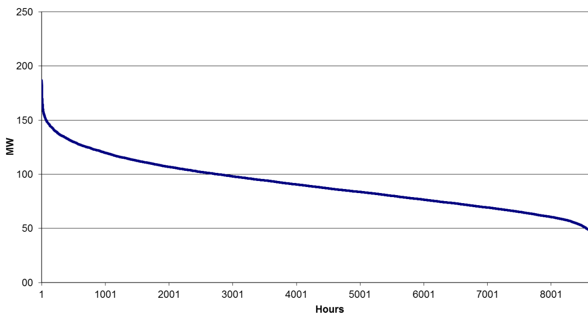
Monotone curve of losses 2017 380-220-150 kV network
