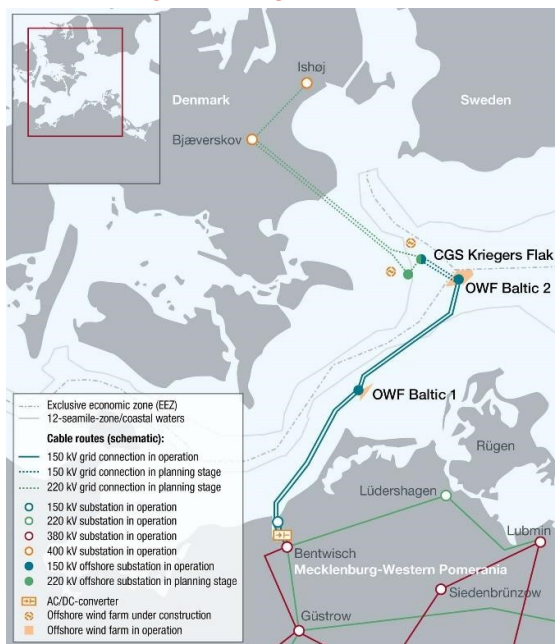
Illustratie 2: Combined Grid Solution
