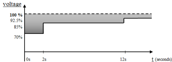
Figure 1: Minimum voltage operating range in black-start conditions
