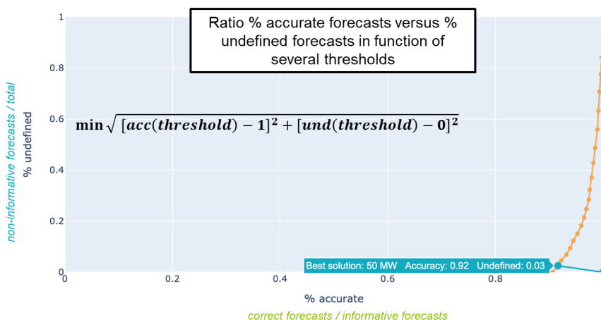
Figure 6 : ratio accurate / undefined forecasts comparing a price-based and flow-based forecasts for different thresholds (up) and methodology to determine the threshold in view of a multi-objective optimization (lower)
