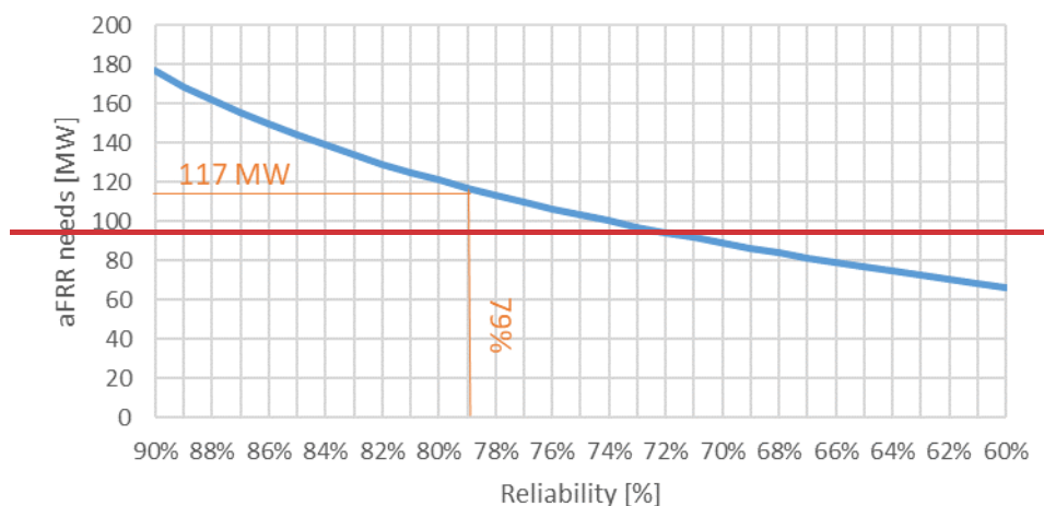
Figure 10 - inverse cumulative probability distribution of the LFC block imbalance variations after imbalance netting
