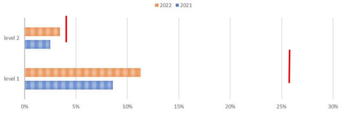
Figure 10 : Elia’s historic performance on FRCE target parameters as specified in Article 128 (legal requirement)
