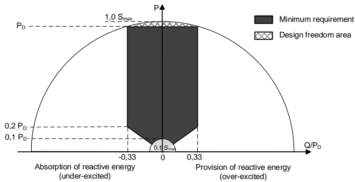
Capability curve for SPGM type B
