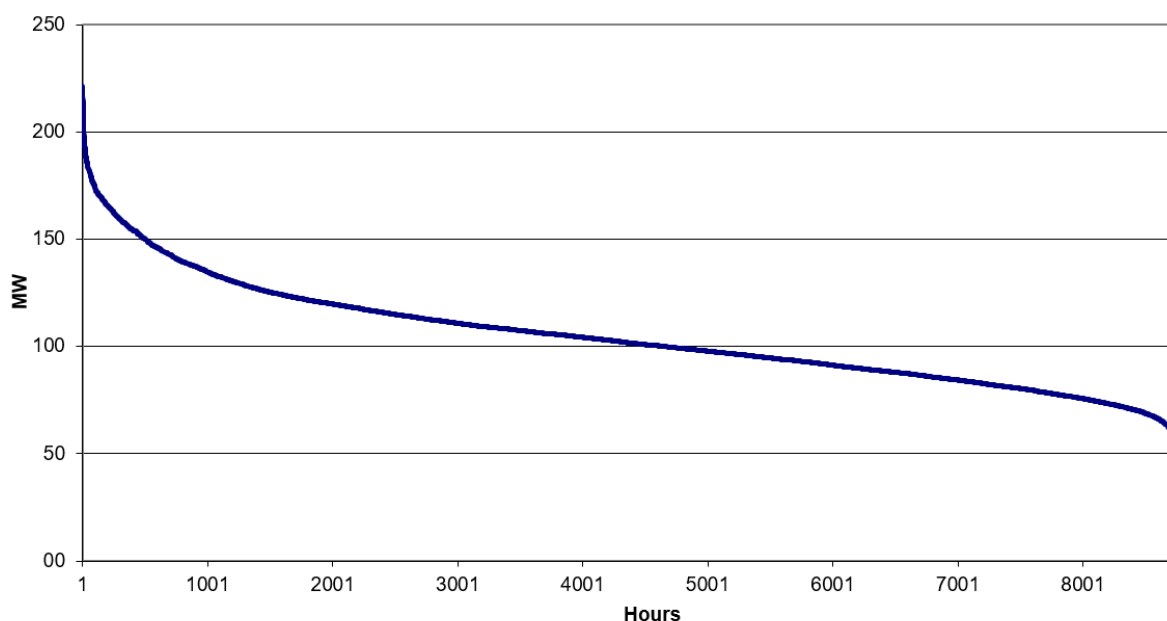
Monotone curve of losses 2021 380-220-150 kV network
