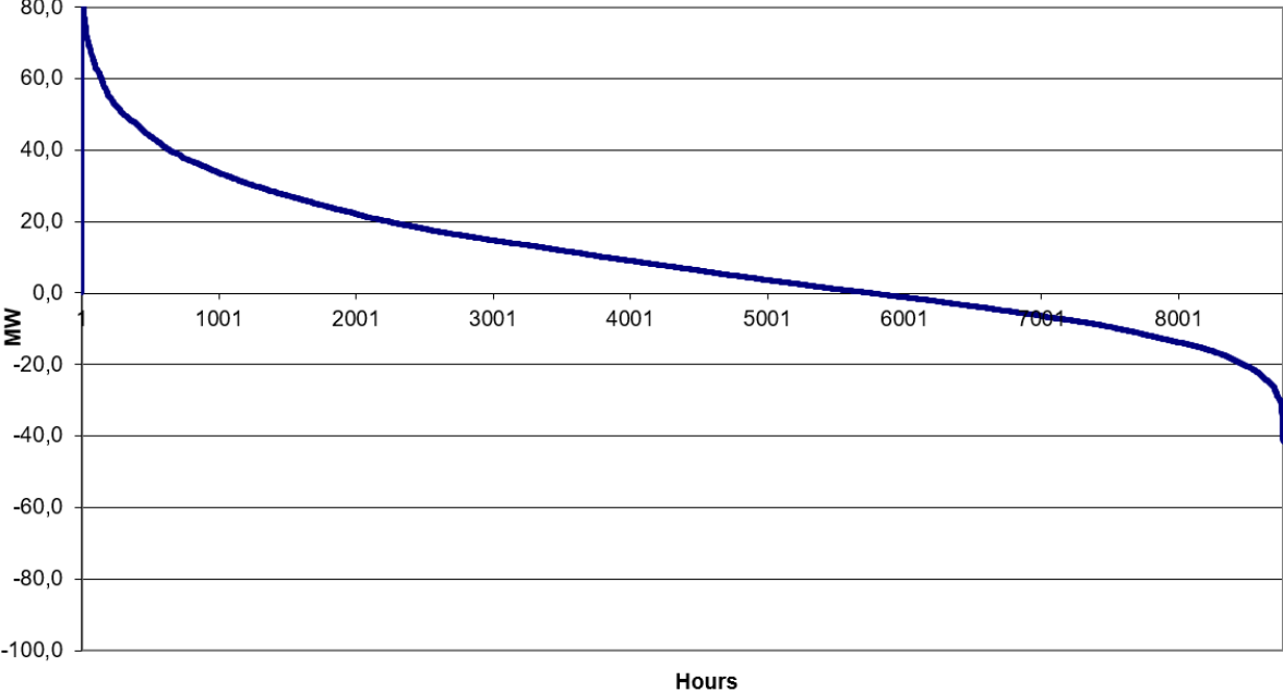
Monotone curve for compensation deficit 2021
