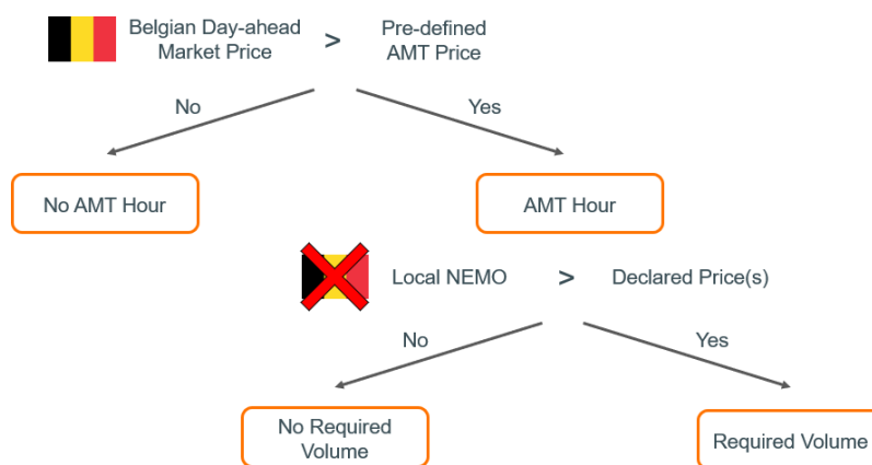
Figure 4 - Flowchart to determine the Required Volume
