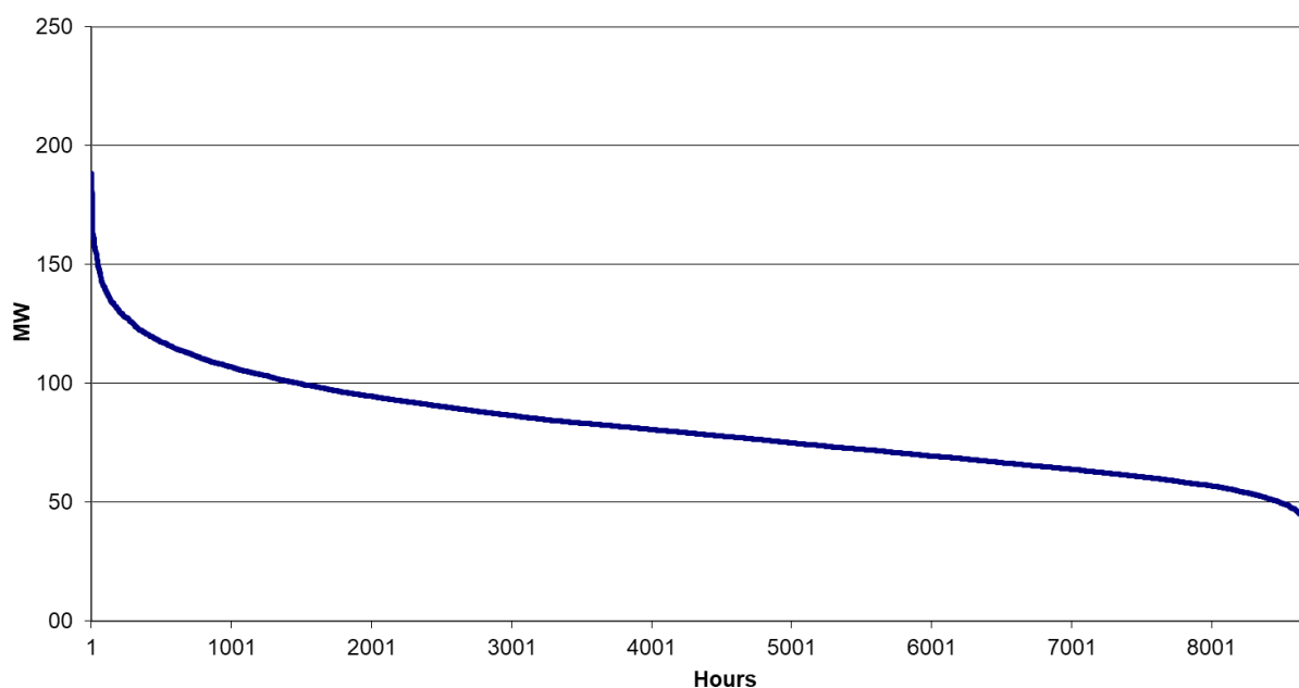
Monotone curve of losses 2020 380-220-150 kV network
